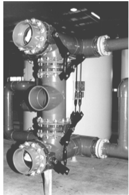
Single linkage available for multiple tank configuration
